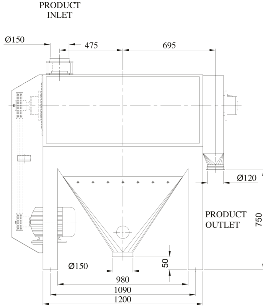
OUTLET OF SIFTED PRODUCT
